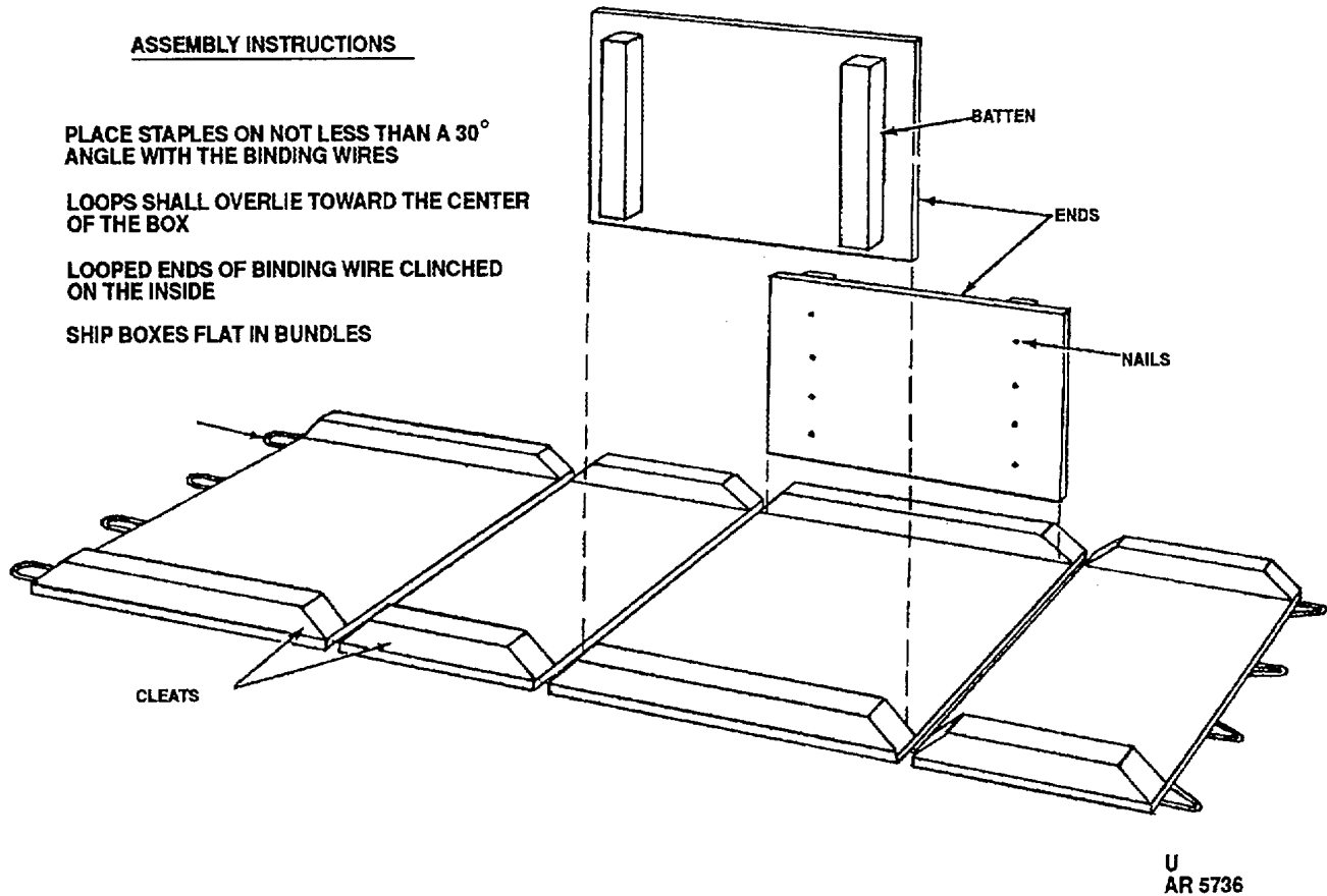
Figure 4-1. Box, wirebound.
