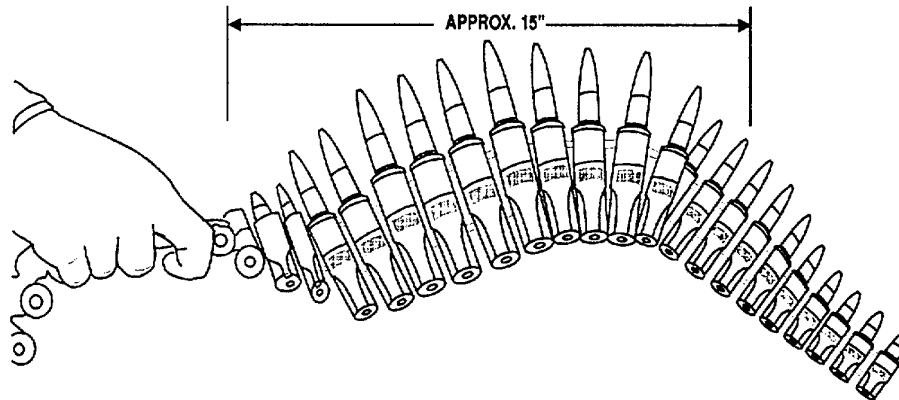
Figure 3-1. Twist inspection.
