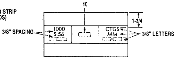
MARKING ON END OF BOX (2 PLACES)
